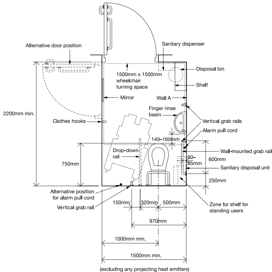
Diagram 18 Unisex wheelchair-accessible toilet with corner WC
